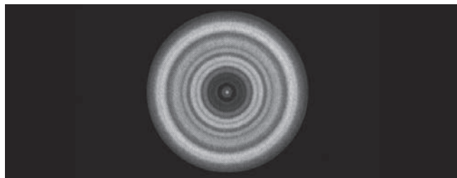
OUT-OF-FOCUS STAR IMAGE FOR COLLIMATED TELESCOPE
